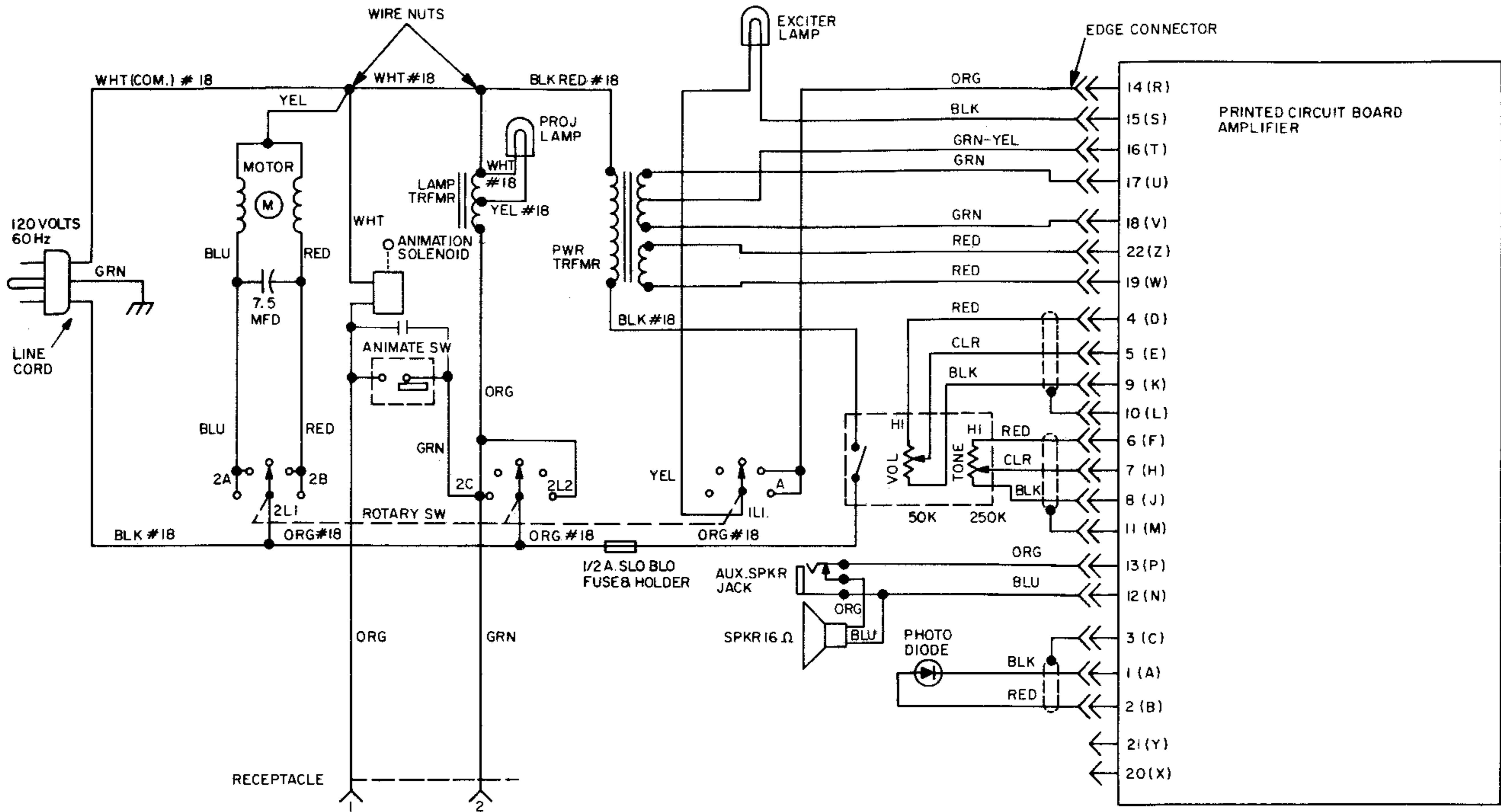
PROJECTOR SCHEMATIC DIAGRAM
