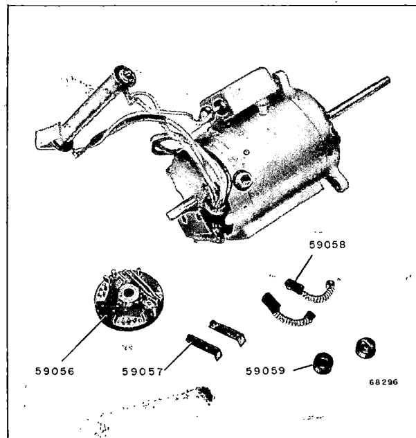
Figure 2—Motor and Replacement Parts
