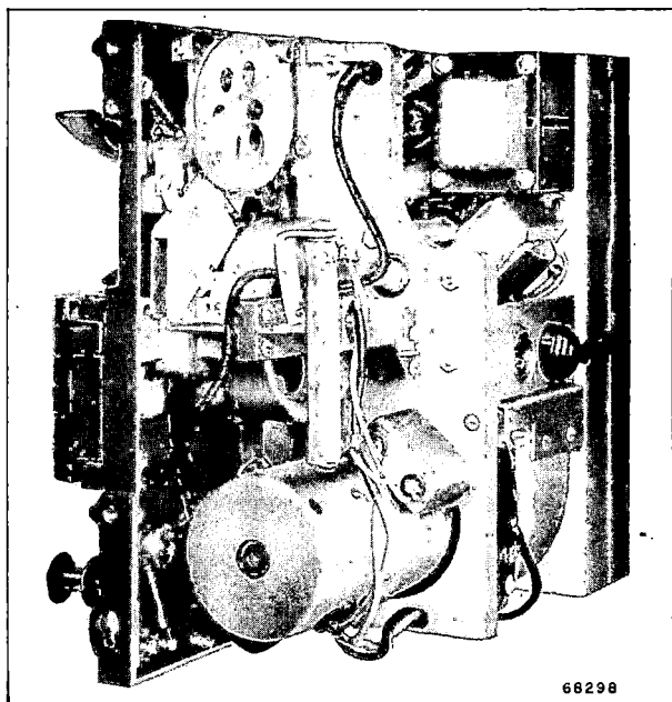
Figure 1—Motor Installed
